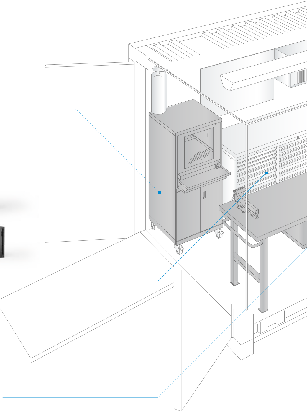
Drawer cabinets variable and flexibly configurable cabinet and drawer size, equipment, locking system and colour, drawers with a load capacity of up to 200 kg
